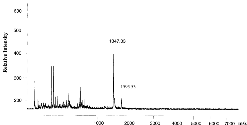
FIG. 6. Matrix assisted laser desorption ionization time of flight (MALDI-TOF) mass spectrometry analysis of the Lys-C-derived, amino-terminal blocked peptide of \beta FGF-1. The peak labeled 1595.53 m/z represents the ovine FGF-1 fraction, while the peak labeled 1347.33 m/z is the Substance P internal standard. The remaining peaks are due to the DHB matrix.
